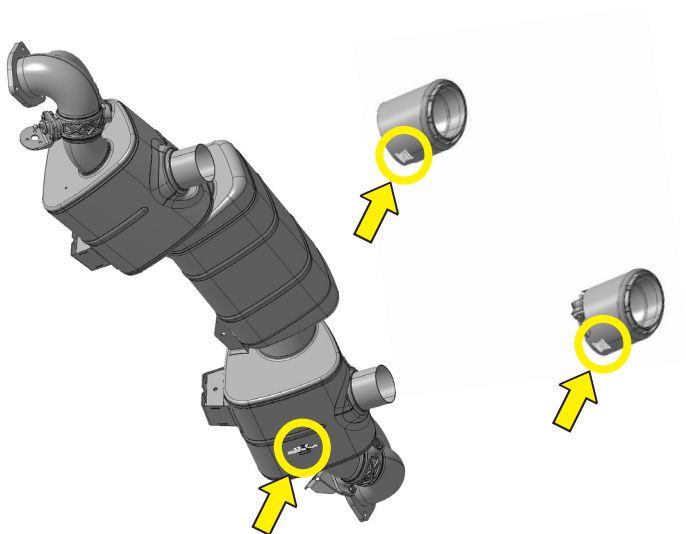
Picture 1 - SERIAL NUMBER POSITIONS:
